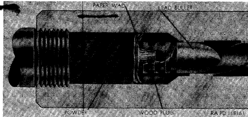
Fig 3 Expanding Bullet as Loaded in Gun
